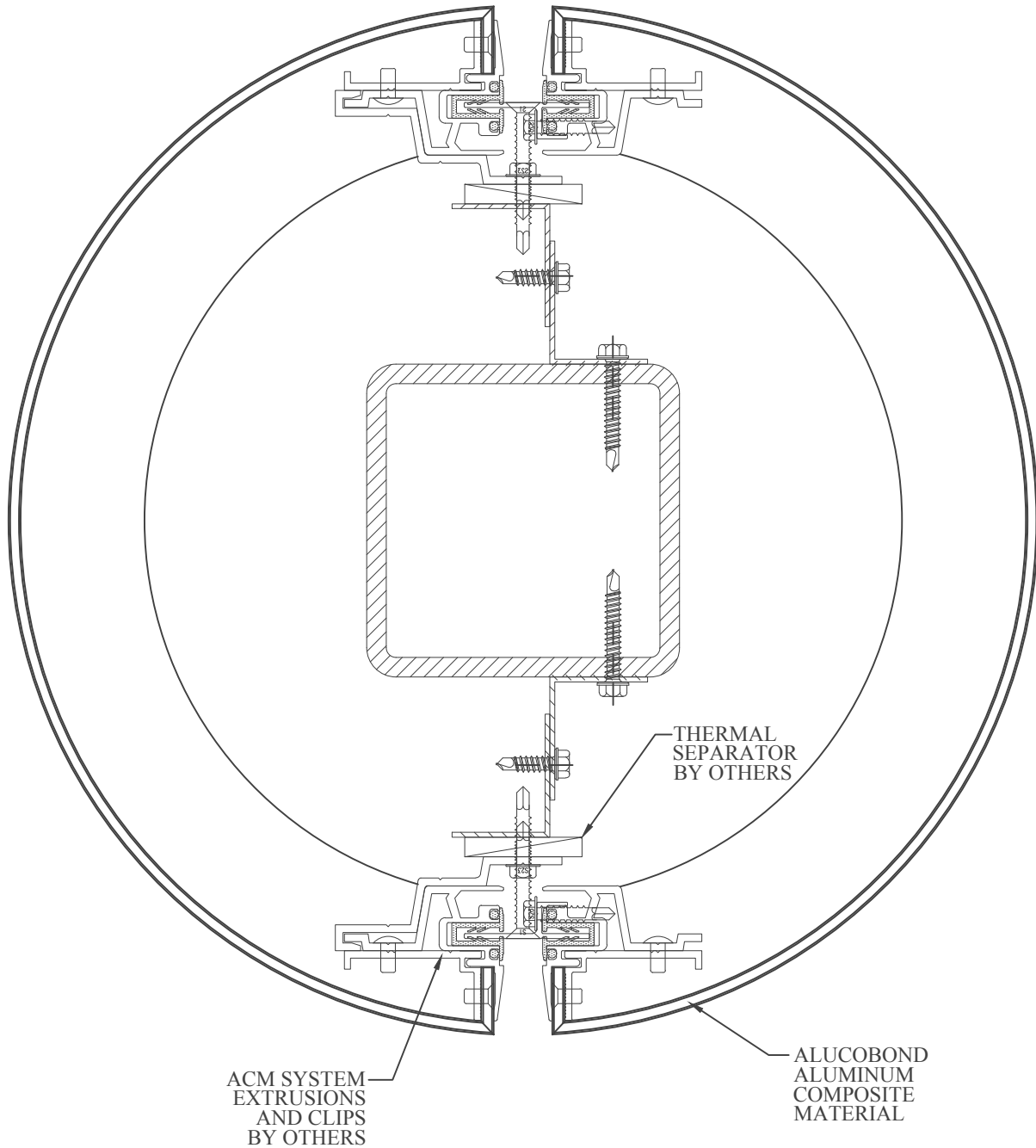
⑮ RADIUS COLUMN DETAIL
