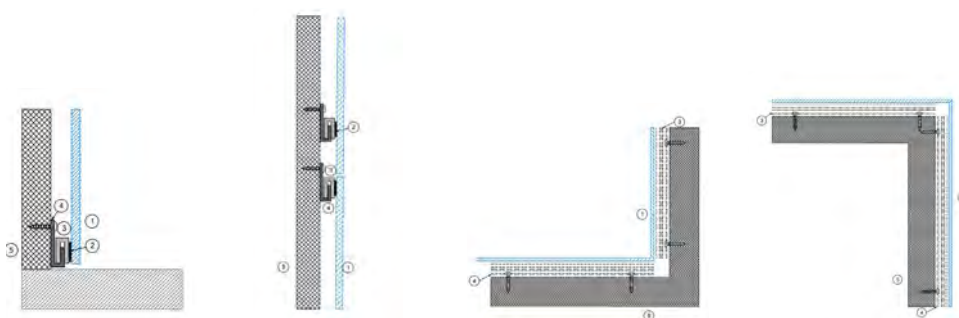
Base Detail
