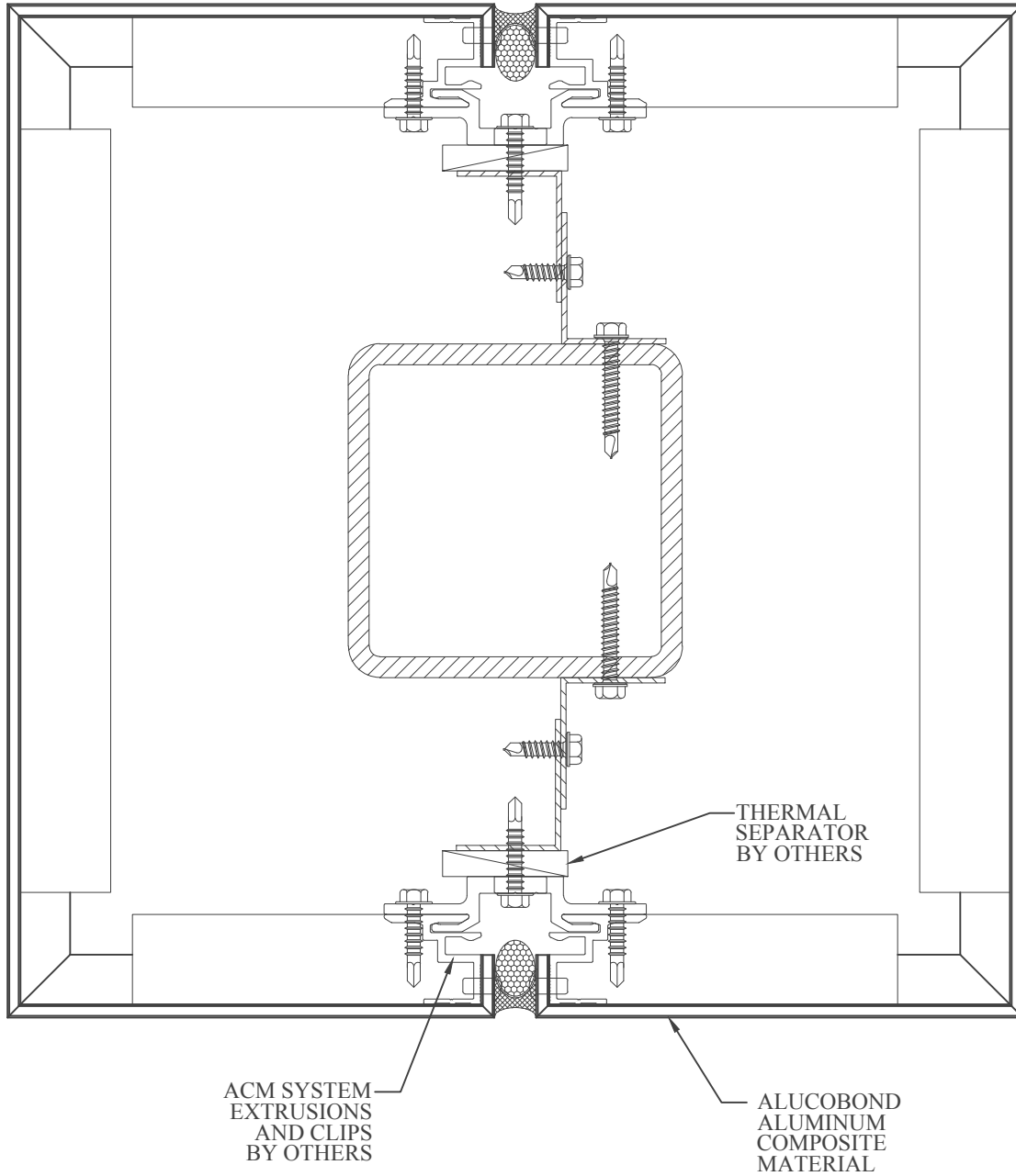
13 SQUARE COLUMN DETAIL
