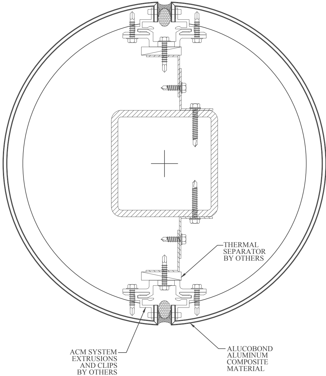
14 RADIUS COLUMN DETAIL
