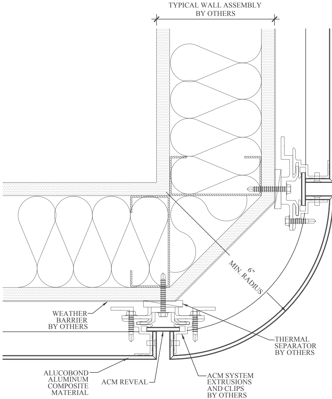
⑫ RADIUS OUTSIDE CORNER DETAIL
