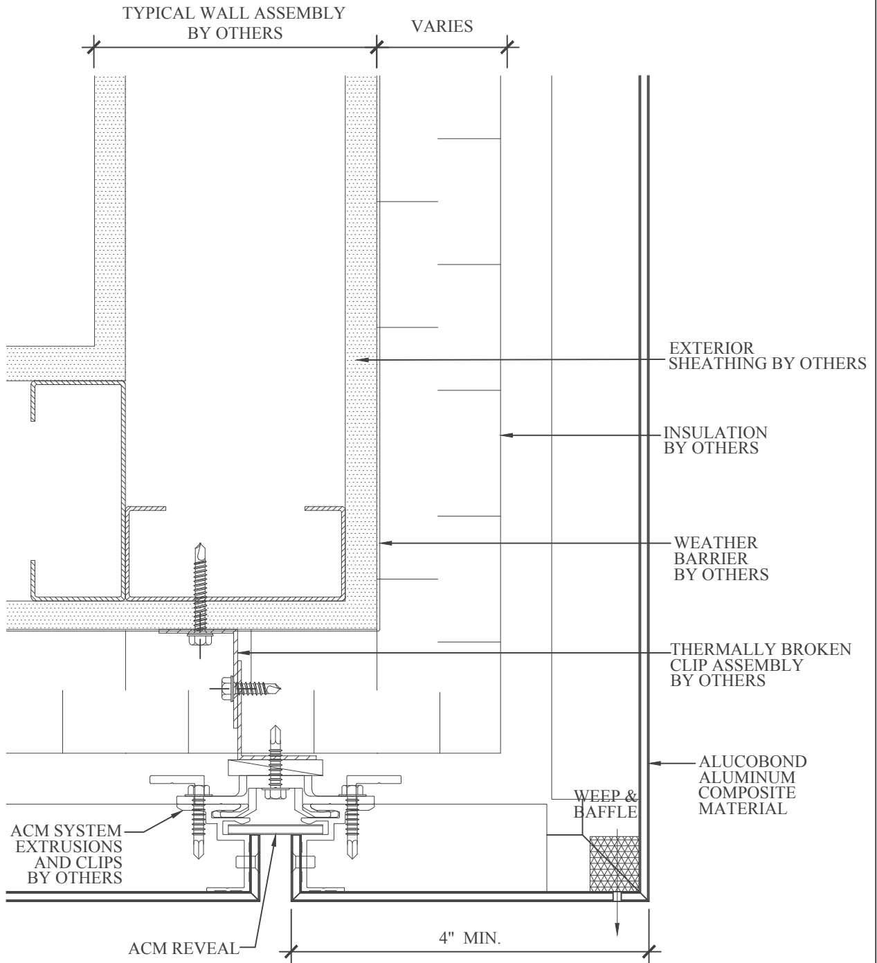
5 WALL/SOFFIT TRANSITION DETAIL
