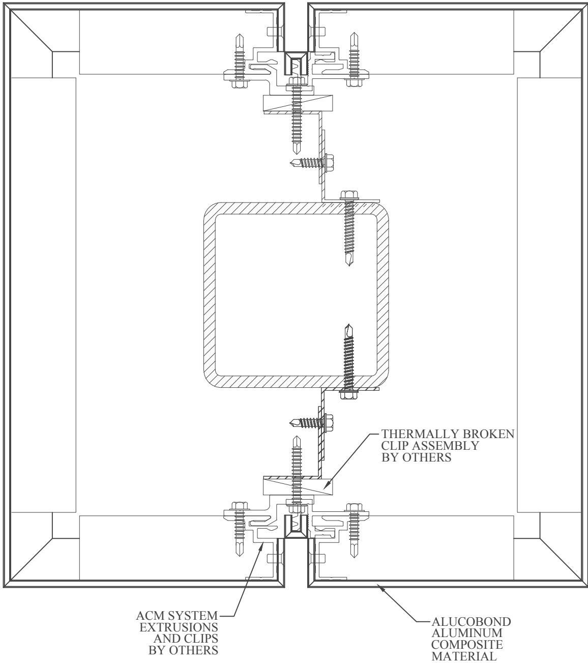
14 SQUARE COLUMN DETAIL
