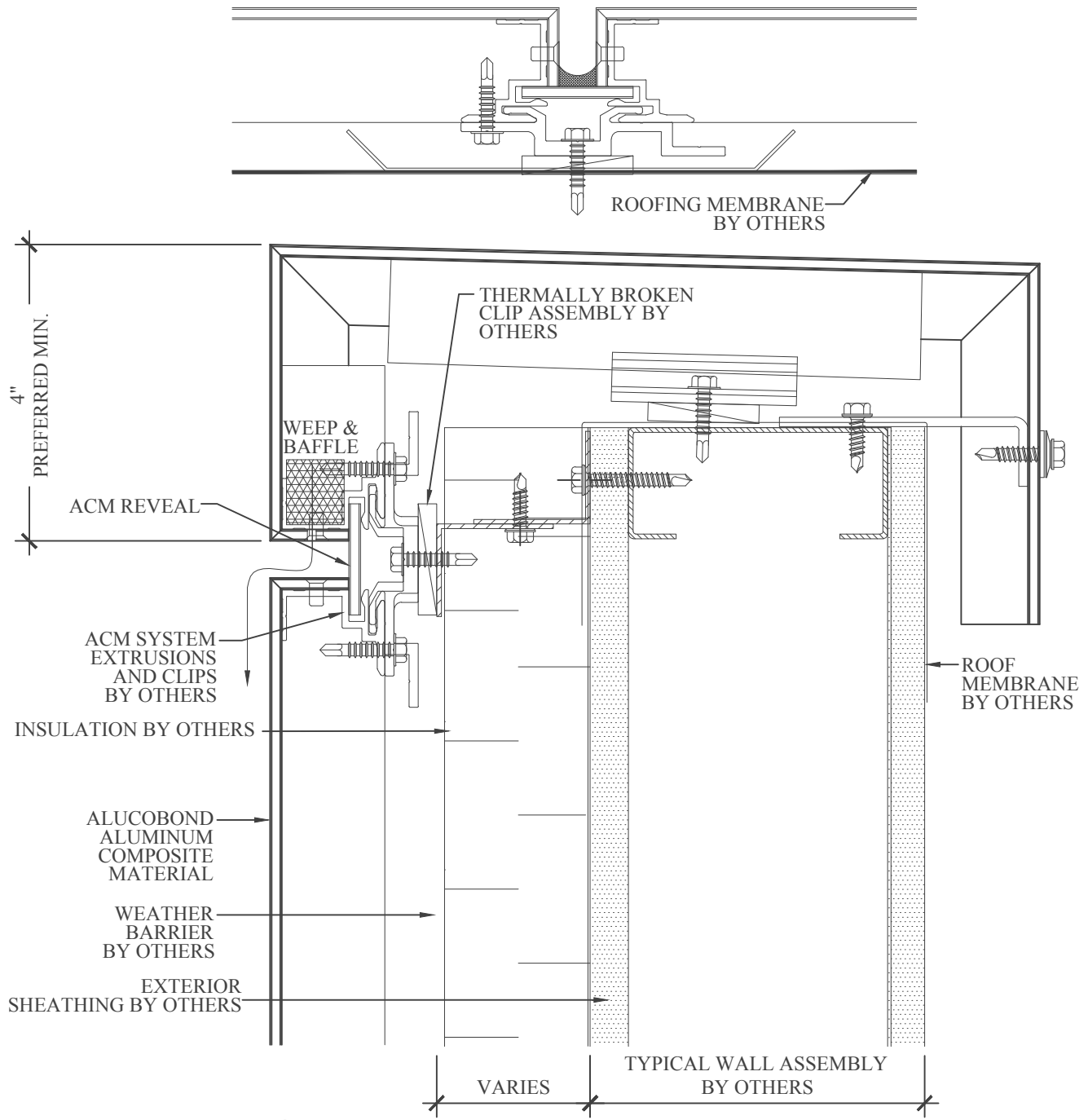
① PARAPET CONDITION DETAIL
