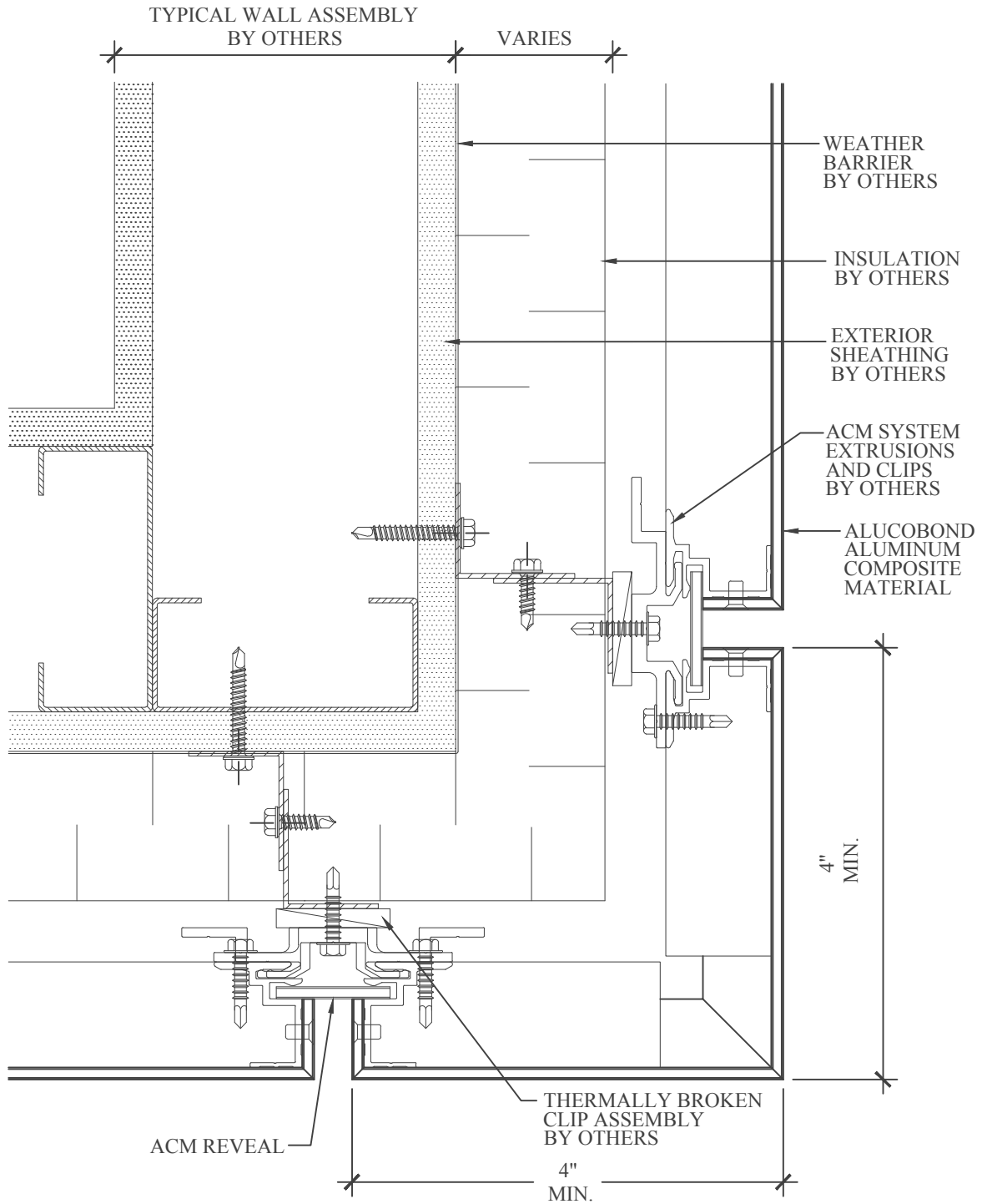
9 OUTSIDE CORNER DETAIL
