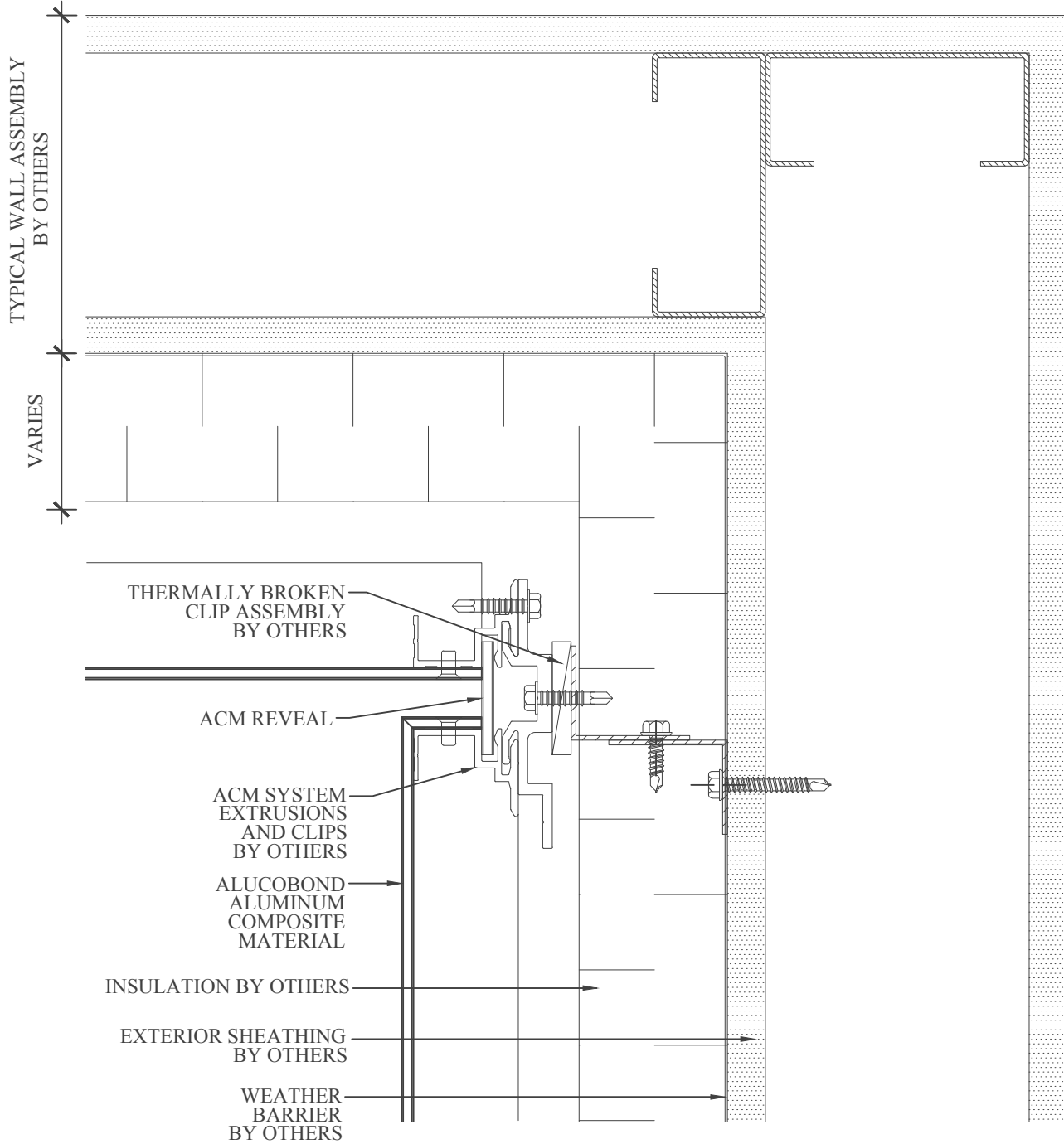
⑪ INSIDE CORNER DETAIL
